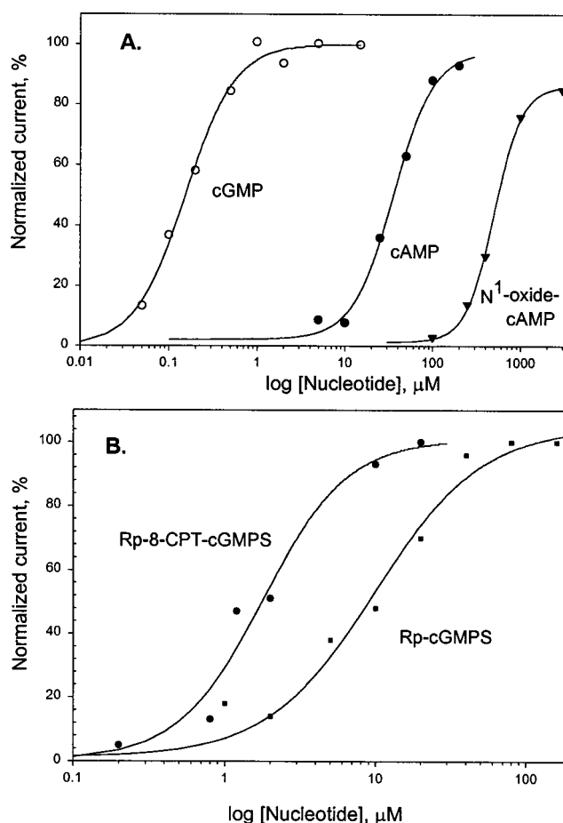
FIGURE 2 ( A ) Activation of the rat olfactory CNG channel by cGMP, cAMP, and N^1 -oxide cAMP. Normalized currents for cGMP (○), cAMP (●), and N^1 -oxide cAMP (▼) are plotted at +60 \text{ mV} with the Hill fits to the data indicated by the solid line. The K_{0.5} for cGMP was 0.14 \mu\text{M} with n_H = 1.5 , the K_{0.5} for cAMP was 35.6 \mu\text{M} with n_H = 1.9 , and the values for N^1 -oxide cAMP were 619 \mu\text{M} and 3.9 , respectively. Averaged values for the K_{0.5} and n_H were 0.54 \mu\text{M} and 1.14 ( n = 4 ) for cGMP, 54 \mu\text{M} and 2.0 ( n = 3 ) for cAMP, and 656 \mu\text{M} and 2.5 ( n = 3 ) for N^1 -oxide cAMP. ( B ) Activation of the rat olfactory CNG channel by Rp-cGMPS isomers. Normalized currents were plotted as a function of nucleotide concentration. The solid lines indicate the Hill fits. Rp-cGMPS (●) had a K_{0.5} of 10.6 \mu\text{M} with an n_H of 1.2 , and Rp-8-CPT-cGMPS (▼) had a K_{0.5} of 1.8 \mu\text{M} with an n_H of 1.6 .
